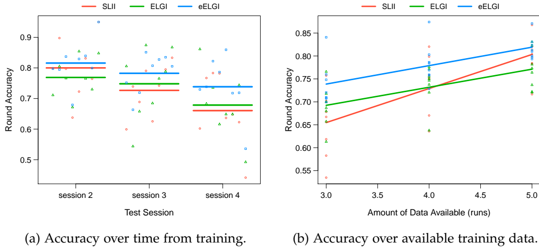
Figure 7.6: Fit of hierarchical linear models, with random effects for each participant, estimating (a) the overall Round Accuracy per testing set and (b) the change in Round Accuracy over training set size.
