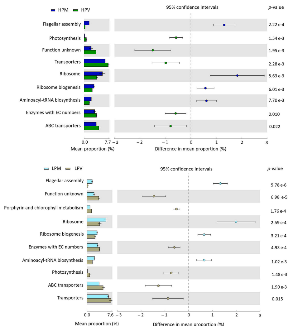
Fig. 9. Predictive functional analysis of bacterial communities (PICRUSt) of group T0.
