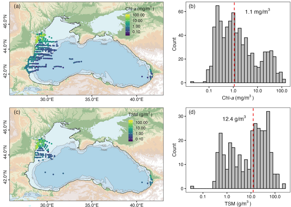
Figure 3. Chl-a and TSM distributions in the in situ dataset. (a) Map of in situ Chl-a, (b) histogram of in situ Chl-a, (c) map of in situ TSM, and (d) histogram of in situ TSM. The red dashed line in the histogram plots represents the median value of Chl-a and TSM.
