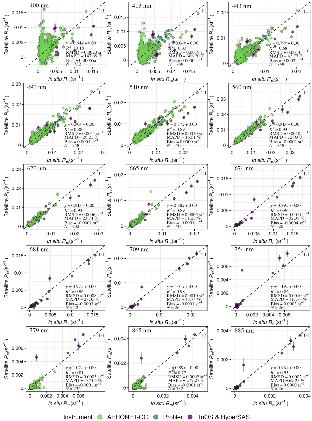
Figure 5. Validation of R_{rs} for CMEMS OLCI products. The vertical bars represent one standard deviation within the 3 × 3-pixel window. The color represents the instrument (or platform) used for measuring R_{rs} . Bands at 754 nm and 885 nm are produced internally but not distributed by CMEMS.
