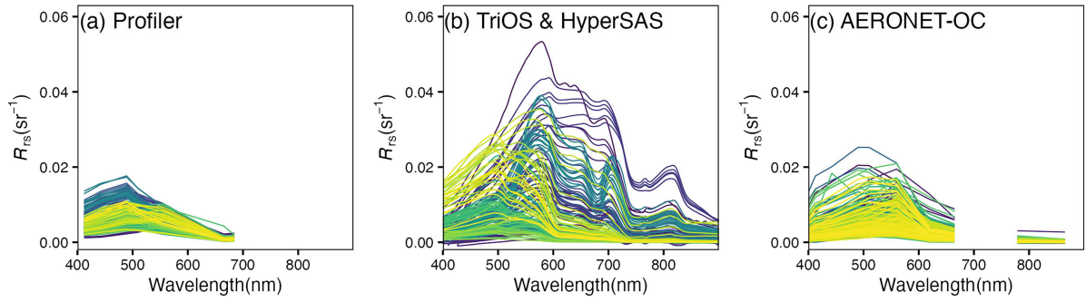
Figure 2. Remote sensing reflectance ( R_{rs} ) spectra collected from (a) Profiler, (b) TriOS and HyperSAS, and (c) AERONET-OC sites in the Black Sea. The color indicates the spectra from different stations or dates.
